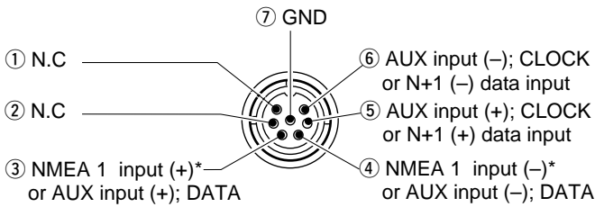
NMEA1 connection
