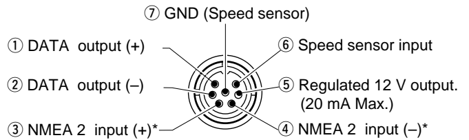
NMEA2 connection
