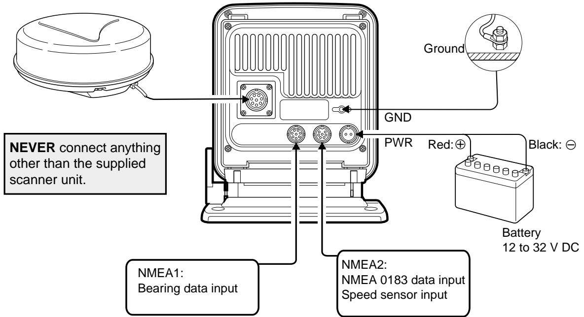
NMEA1 connection
